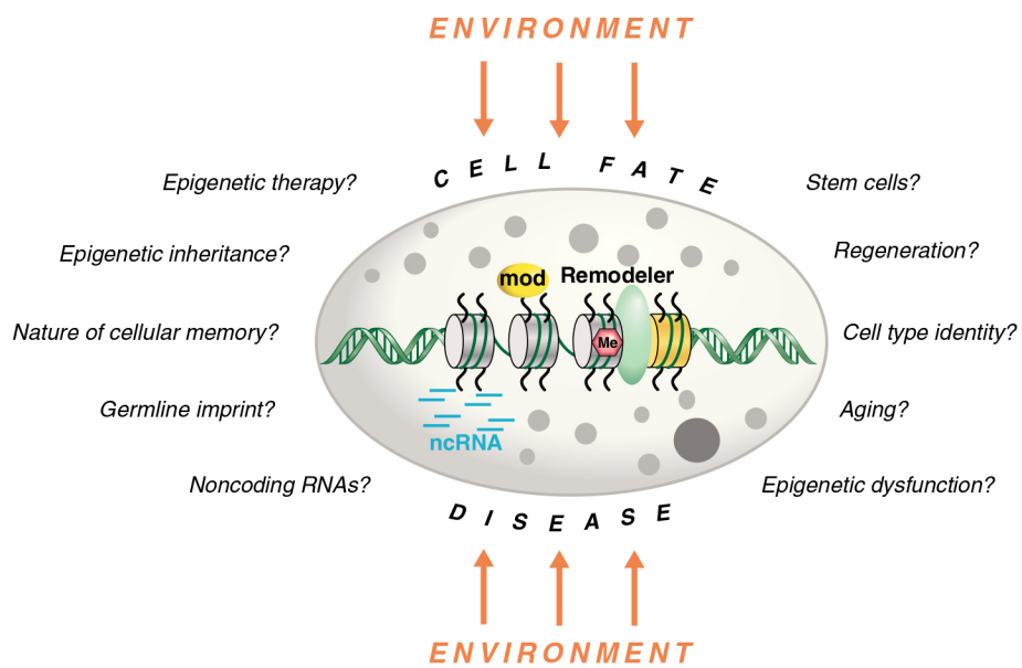
Figure 38. Big questions in epigenetic research. The many experimental systems used in epigenetic research have unveiled numerous pathways and novel insights into the mechanisms of epigenetic control. Many questions, as shown in the figure, still remain and require further elucidation or substantiation in new and existing model systems and methods.
